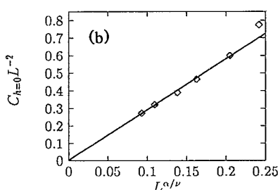
FIG. 5. (a) Plot of \log -\frac{\partial \Delta F}{\partial t} \big|_{t=0} vs \log L . The line is a least-squares fit to the data points. The slope of the line gives \nu \approx 1.40 . (b) Plot of C_{h=0}L^{-2} vs L^{\alpha/\nu} with \alpha/\nu = 2/\nu - 2 = -0.57 at t = 0 .
